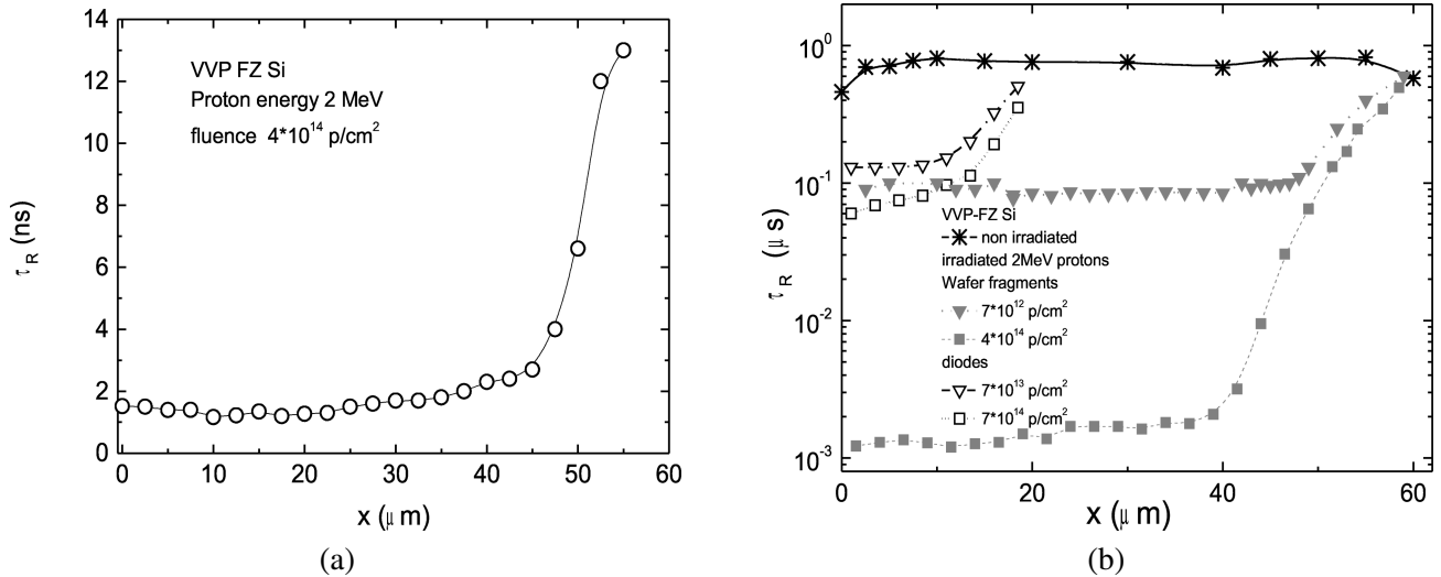
Fig. 4. (a) Recombination lifetime in-depth variation within n -Si substrate layer irradiated with 2 MeV protons and 4 \cdot 10^{14} p/cm 2 fluence, and (b) comparison of the absolute values of recombination lifetime and its depth-profiles measured by MW-PC cross-sectional scans in n -Si layer of substrate as well as of diode base irradiated by 2 MeV proton beam at various fluences relatively to non-irradiated material.
