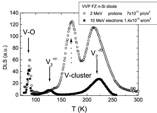
Fig. 6. Comparison of the DLTS spectra measured in diodes irradiated with 10 MeV electrons and 2 MeV protons of nearly the same fluence (around 10^{13} \text{ cm}^{-2} ).
