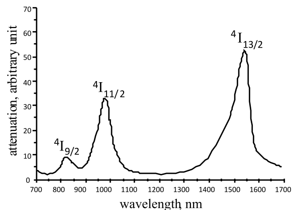
Fig. 1. Absorption spectrum of an erbium doped silica fiber [3].
