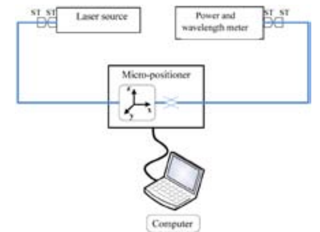
Fig. 2. The block diagram of the measurement breadboard.
