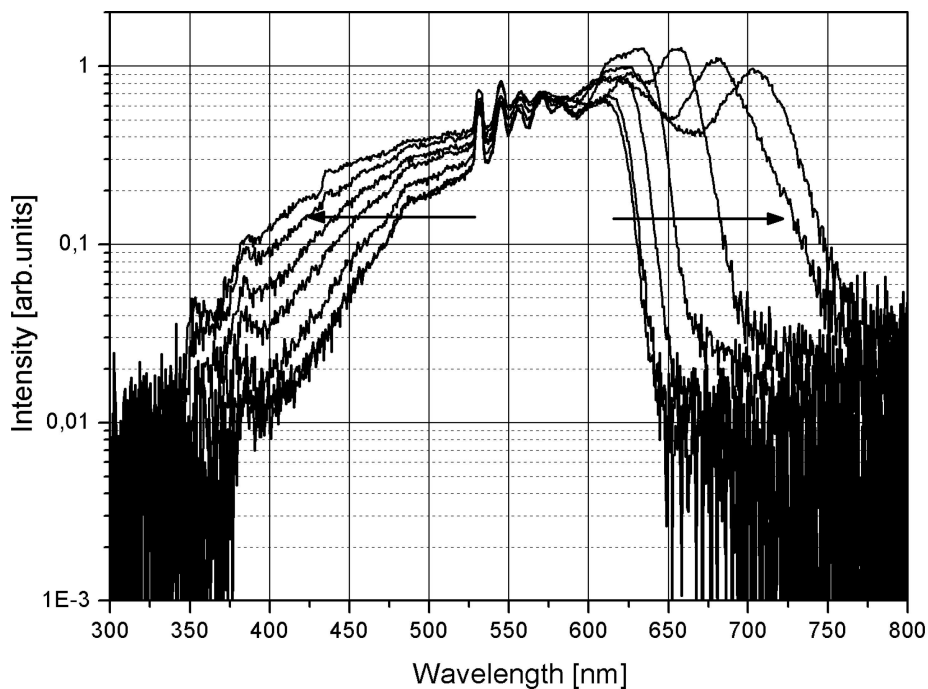
Fig. 8. Dependence of the spectrum of continuum generated at dual wavelength pump on pump power (from 9 to 25 mW and from 1.5 to 5 mW at 1062 nm and 531 nm respectively) for PCF with ZDW at 800 nm. Arrows indicate broadening of continuum spectrum with increasing the pump power.
