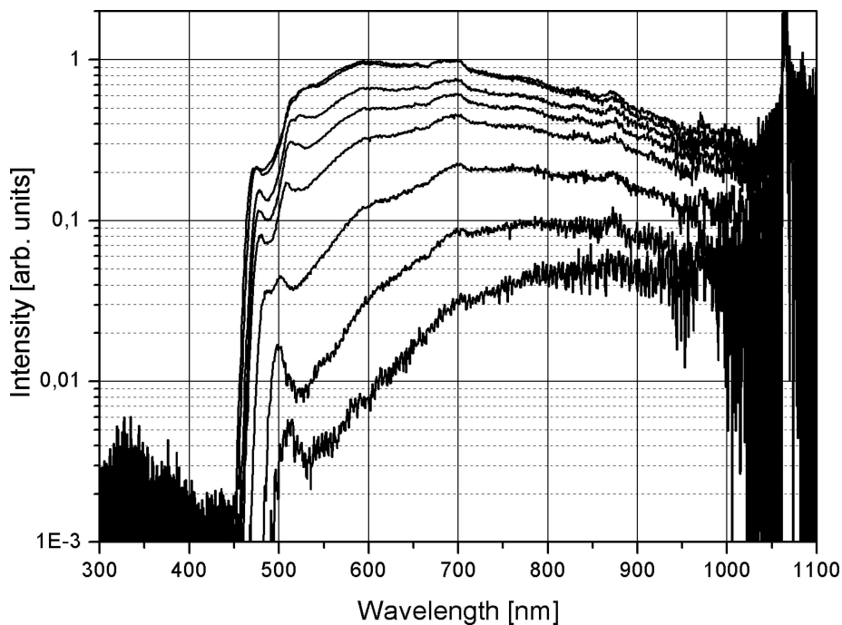
Fig. 6. Dependence of the spectrum of continuum generated in PCF with ZDW at 1040 nm on pump power at 1062 nm (from 9 to 25 mW).
