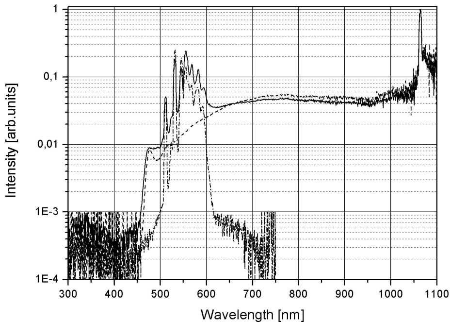
Fig. 5. Spectra of continuum generated in PCF with ZDW at 1040 nm. (---) pump at 1062 nm (pump power 20 mW), (-.-.-) pump at 531 nm (pump power 4 mW), (—) dual-wavelength pump at 1062 nm (pump power 20 mW) and 531 nm (pump power 4 mW).
