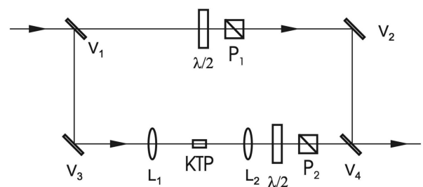
Fig. 3. Experimental set-up for dual-wavelength pump of PCF.
