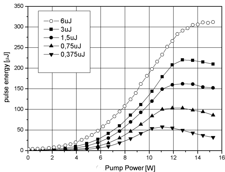
Fig. 2. Dependence of amplified pulse energy on CW laser diode pump power at different energy of seed pulses.
