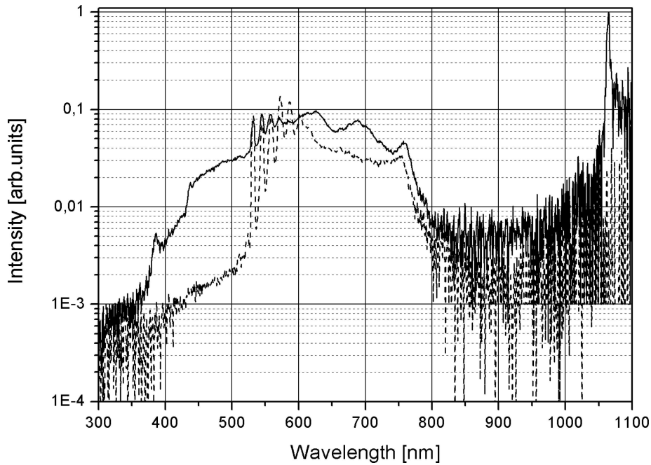
Fig. 7. Spectra of continuum generated in PCF with ZDW at 800 nm. (---) pump at 531 nm (pump power 4 mW), (—) dual-wavelength pump at 1062 nm (pump power 20 mW) and 531 nm (pump power 4 mW).
