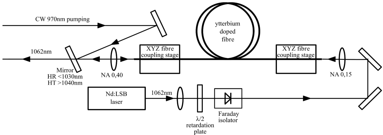
Fig. 1. Experimental set-up of ytterbium doped fibre amplifier.
