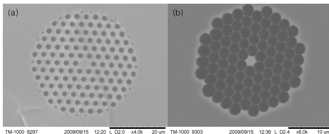
Fig. 4. Cross-section of photonic crystal fibres:(a) with ZDW at 1040 nm, (b) with ZDW at 800 nm.
